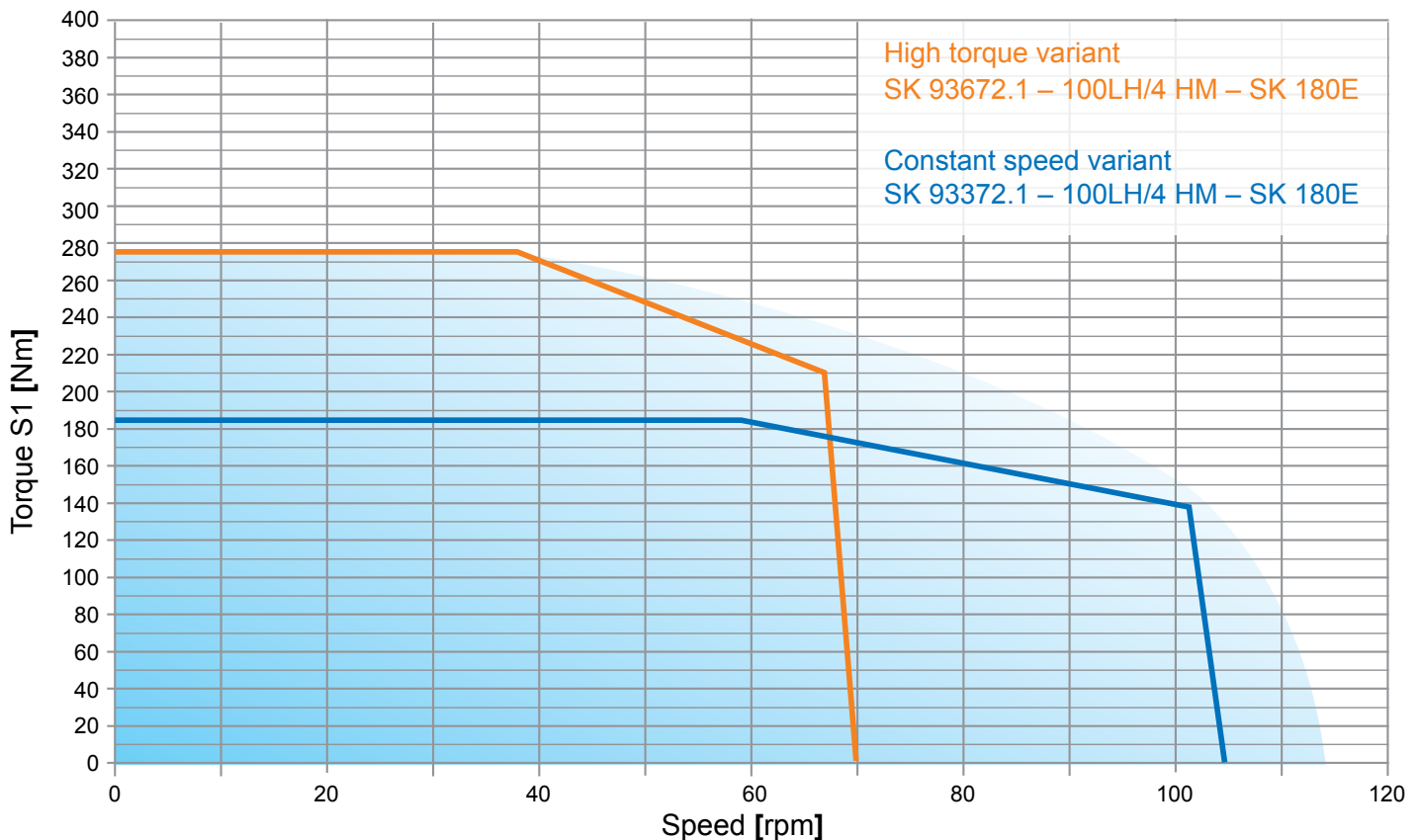
Torque graph
